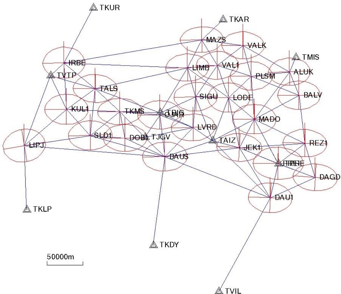
Fig.2. Adjusted GNSS vector scheme
