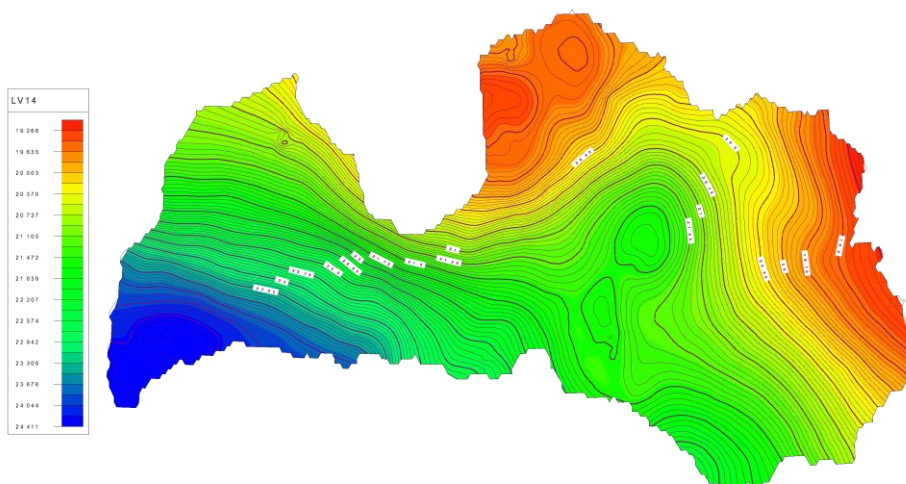
Fig.1. Kvasigeoid model - LV14
