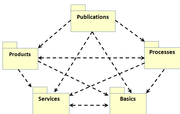
Figure 1 - ProSF Model. Arrows show usage relations between packages
